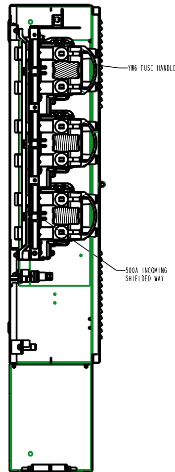
SECTION C-C SHOWING 500A INCOMING SHIELDED FUSEWAY
