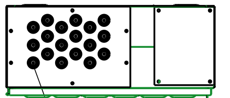
DRILLED STEEL GLANDPLATE WITH CONICAL PLASTIC GROMMETS (3 TO 22.5mm CABLE O/D)
