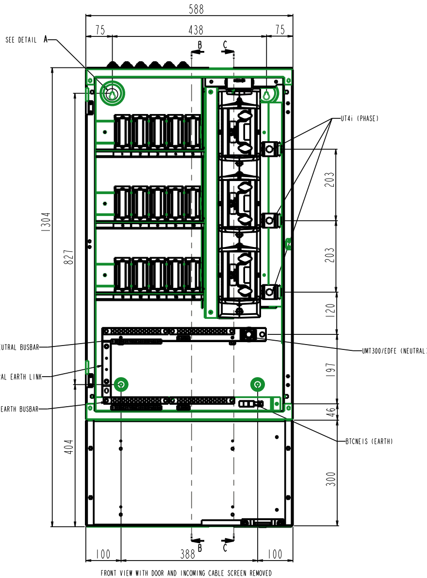
FRONT VIEW WITH DOOR AND INCOMING CABLE SCREEN REMOVED
